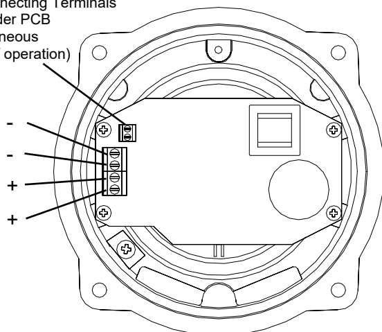
Fig. 5b Beacon DC Terminals
