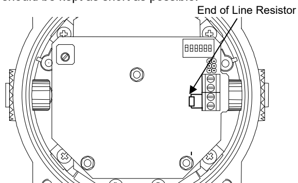
Fig. 7 End of Line Resistor Placement
